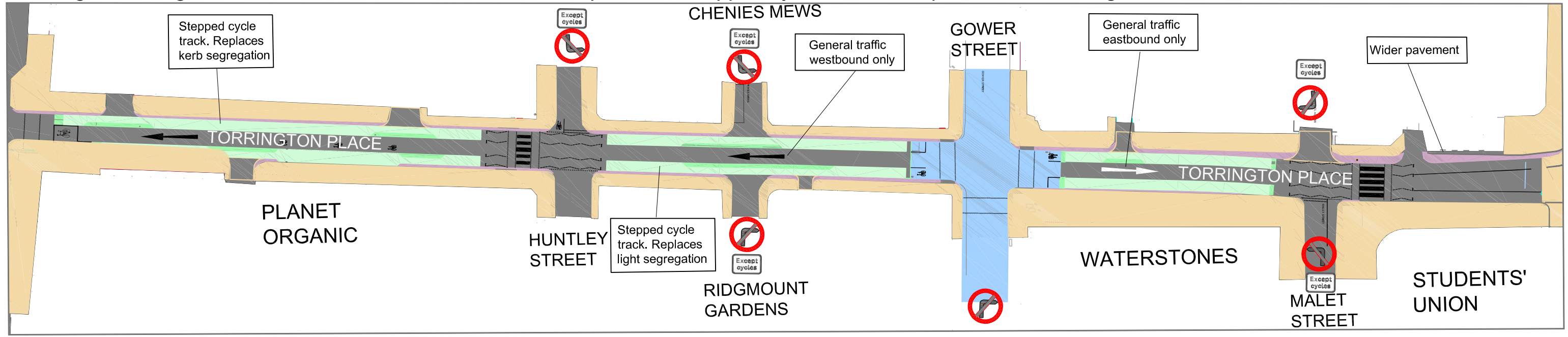
Drawing 3: Torrington Place to Tavistock Place eastbound option with stepped cycle tracks and pavement widening
