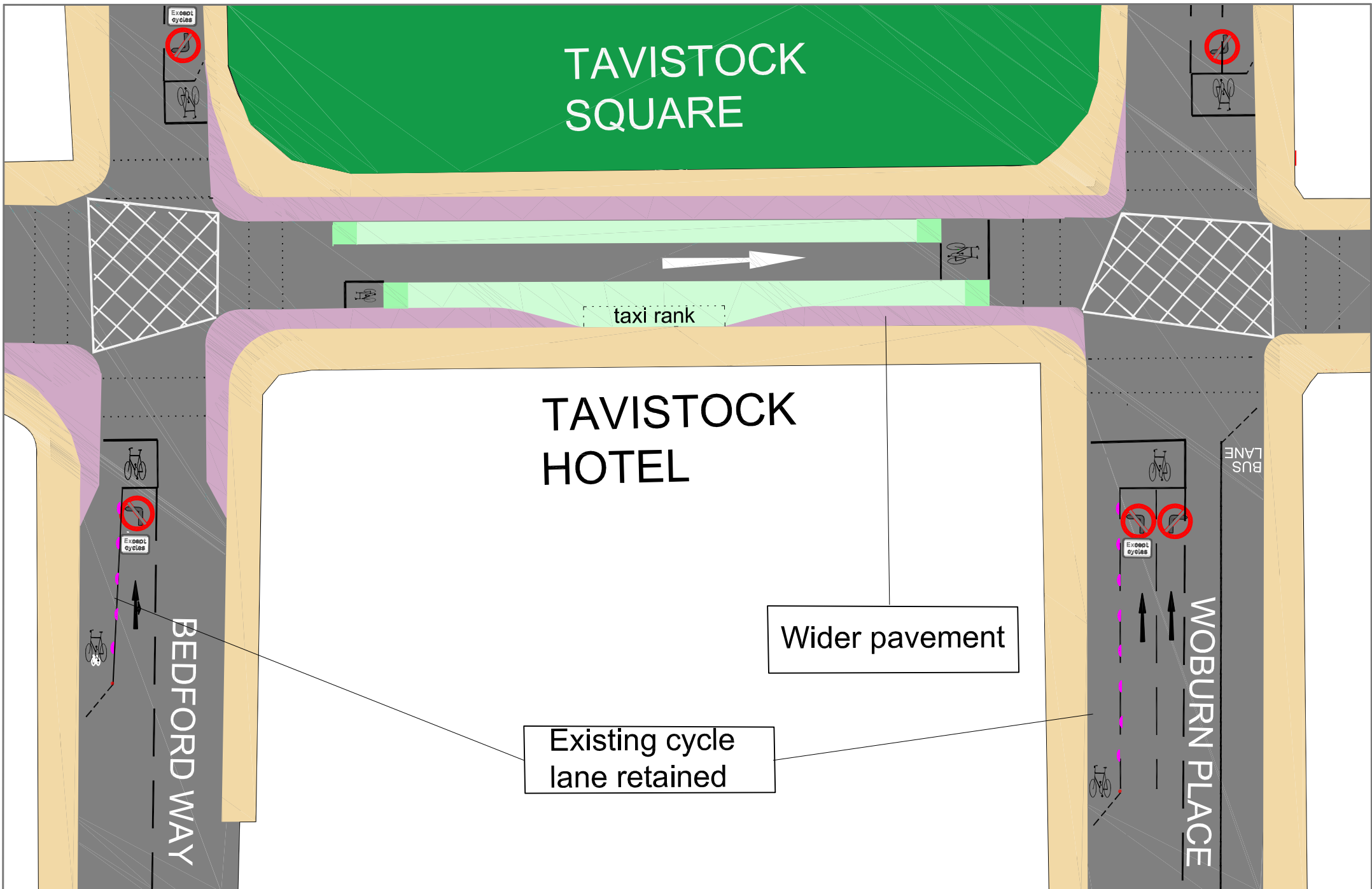
Drawing 3a: Proposals at Bedford Way and Woburn Place junctions with Tavistock Square
